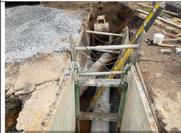
C St NE & 19th St – Excavate and place 15" RCP between M6-10 to I7-3
