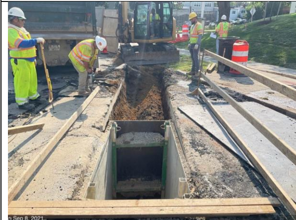
C St NE & 19th St – Excavate 15" RCP between M6-10 to I7-3
