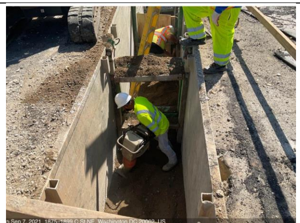
© Sep 7, 2021, 1875-1899 C St NE, Washington DC 20003, US C St NE & 19th St – Backfill 15" RCP between M6-10 to I7-3
